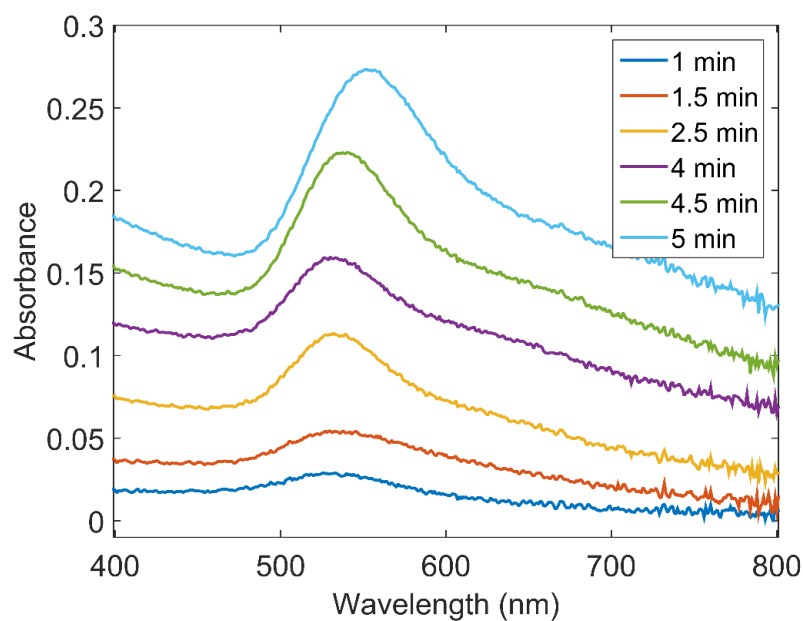
Figure S9. Absorbance as a function of the particle growth time for samples functionalized with DETA 5%.
