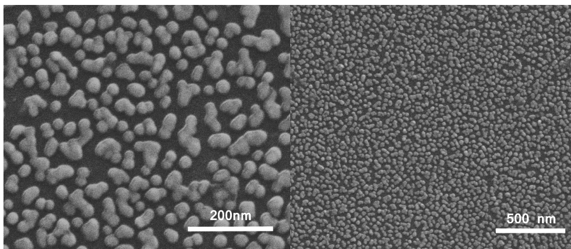
Figure S10. SEM image of growth gold nanoparticles on a APTMS functionalized sample
