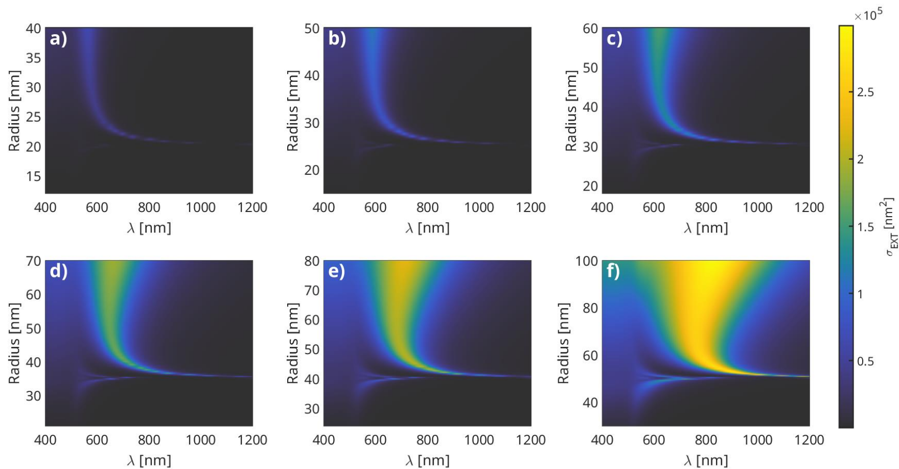
Figure S2. Optical extinction cross sections of gold dimers as a function of light wavelength and particle radius for different center-to-center separation distances d = 40 nm (a), 50 nm (b), 60 nm (c), 70 nm (d), 80 nm (e), and 100 nm (f).
