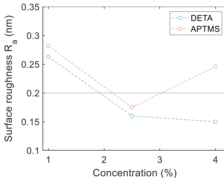
Figure S7. Surface roughness of after the functionalization compared to the roughness of the pristine substrate after cleaning (indicated with the horizontal line at R_a=0.2\text{nm} ).
