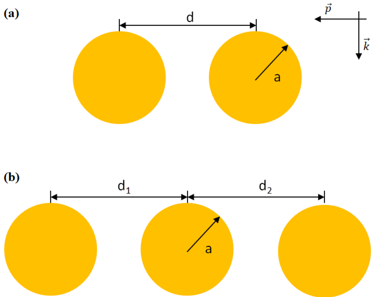
Figure S1. Schematics of the dimer (a) and trimer (b) configurations used in the BEM simulations.
