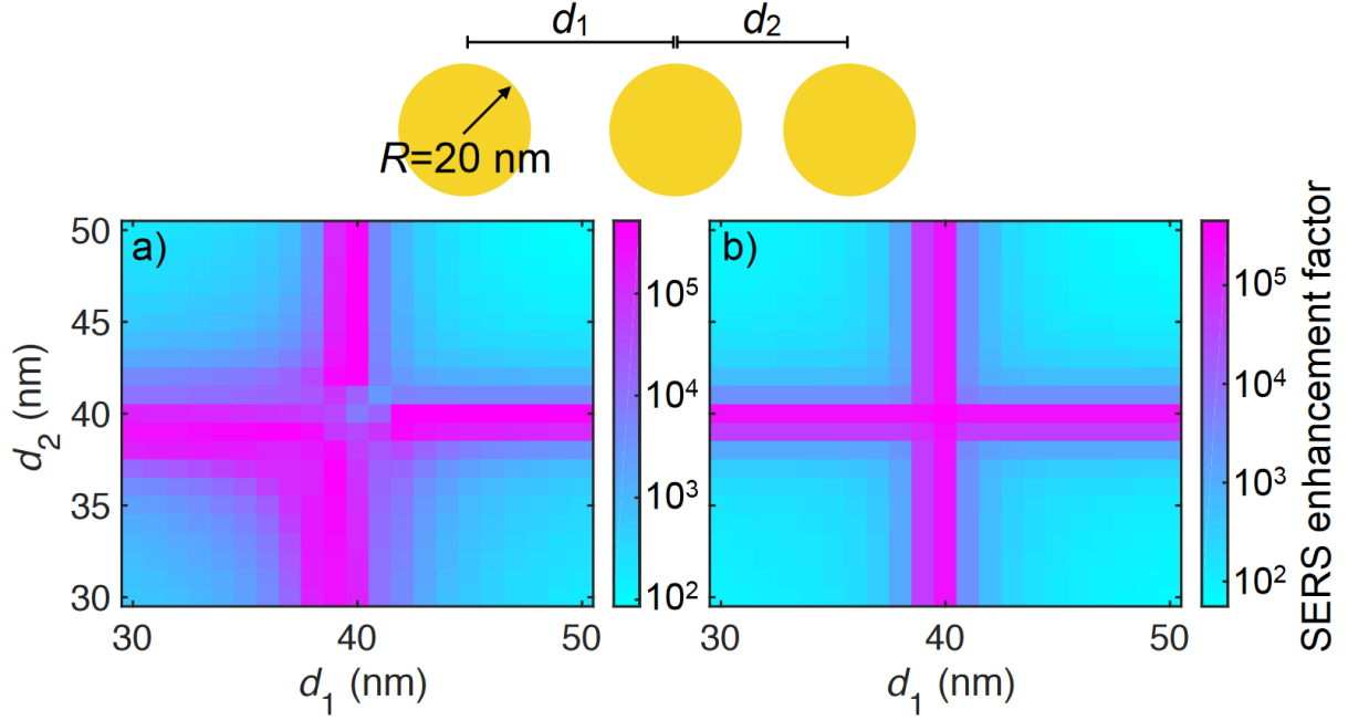
Figure S5. Surface-averaged SERS enhancement factor as a function of two center-to-center separation distances d_1 and d_2 in a gold trimer either directly calculated using boundary-element method (BEM) (a) or constructed by those of two individual dimers (b). Here, we assume an incident light wavelength of 785 nm and a Raman shift of 1380 \text{ cm}^{-1} .
