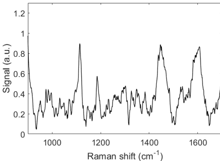
Figure S12. Signal of 100 \mu M Skatole on Klarite under typical acquisition conditions (see Methods).
