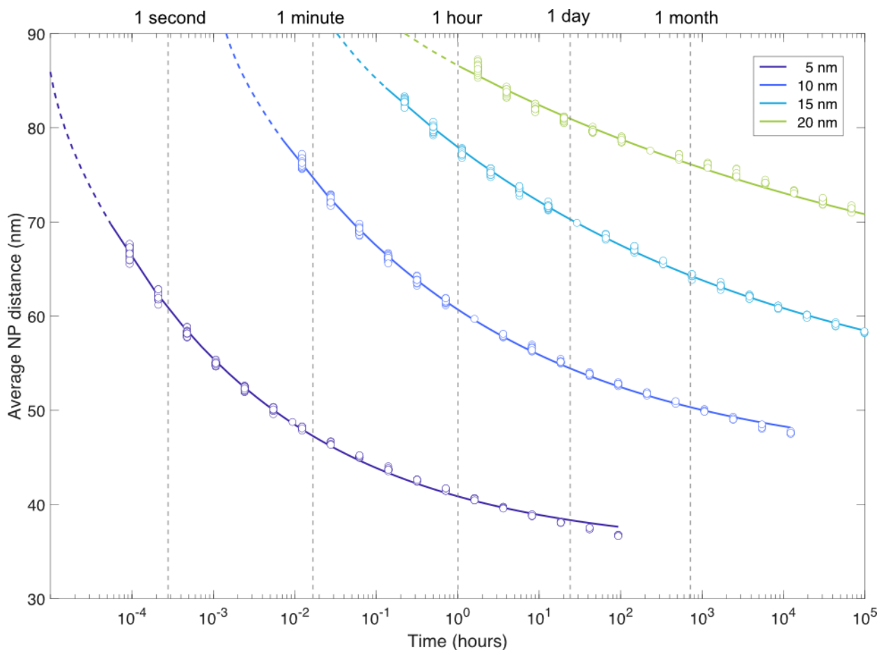
Figure S6. Average nearest neighbor particle distance for different commercially available nanoparticles diameters. The dots represent the data from simulations, and the lines are a guide to the eye.
