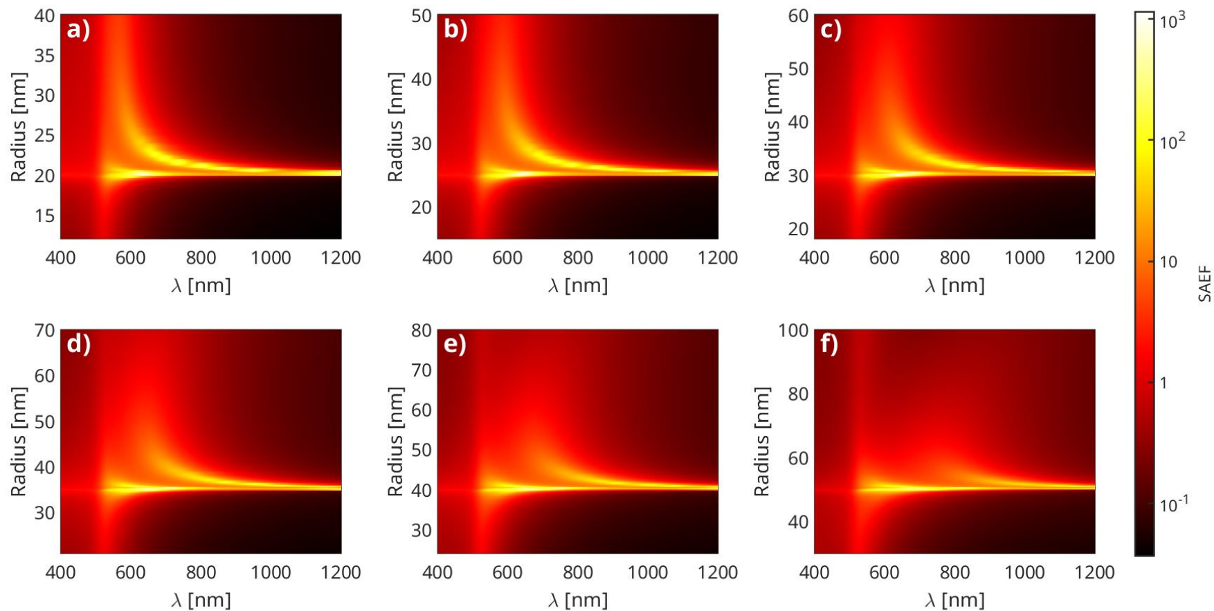
Figure S3. Surface-averaged field intensity enhancement (SAEF) due to the excitation of the plasmonic resonances in gold dimers as a function of light wavelength and the particle radius for different center-to-center separation distances d = 40 nm (a), 50 nm (b), 60 nm (c), 70 nm (d), 80 nm (e), and 100 nm (f).
