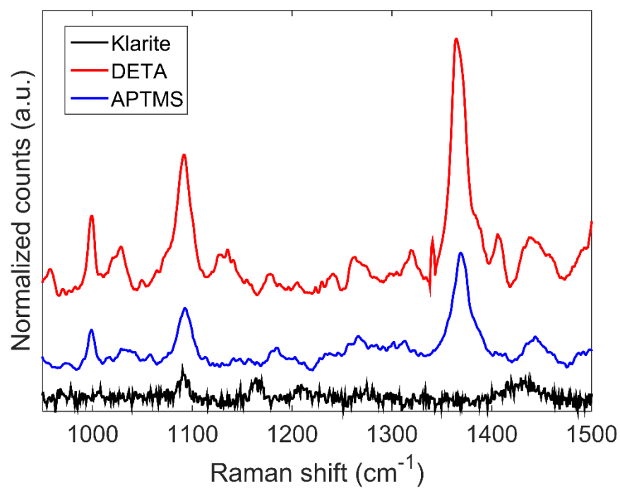
Figure S13. Comparison of SERS signal for Klarite, APTMS 2.5%, and DETA 4% for 10 \mu M Skatole concentration. Measurements were taken under the same conditions in all cases: \lambda=785 nm, power P_{\text{ex}}=100\mu\text{W} , integration time T_{\text{int}}=10\text{s} .
