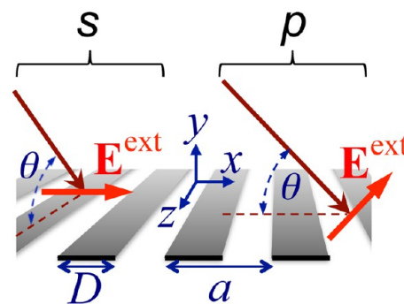
Figure 9. Oblique incidence conditions here considered: external plane wave with wave vector in the yz plane and electric field along x ( s polarization, left); and incident wave vector and external field both in the xy plane ( p polarization, right). Medium 1 (medium 2) is above (below) the ribbon array.
