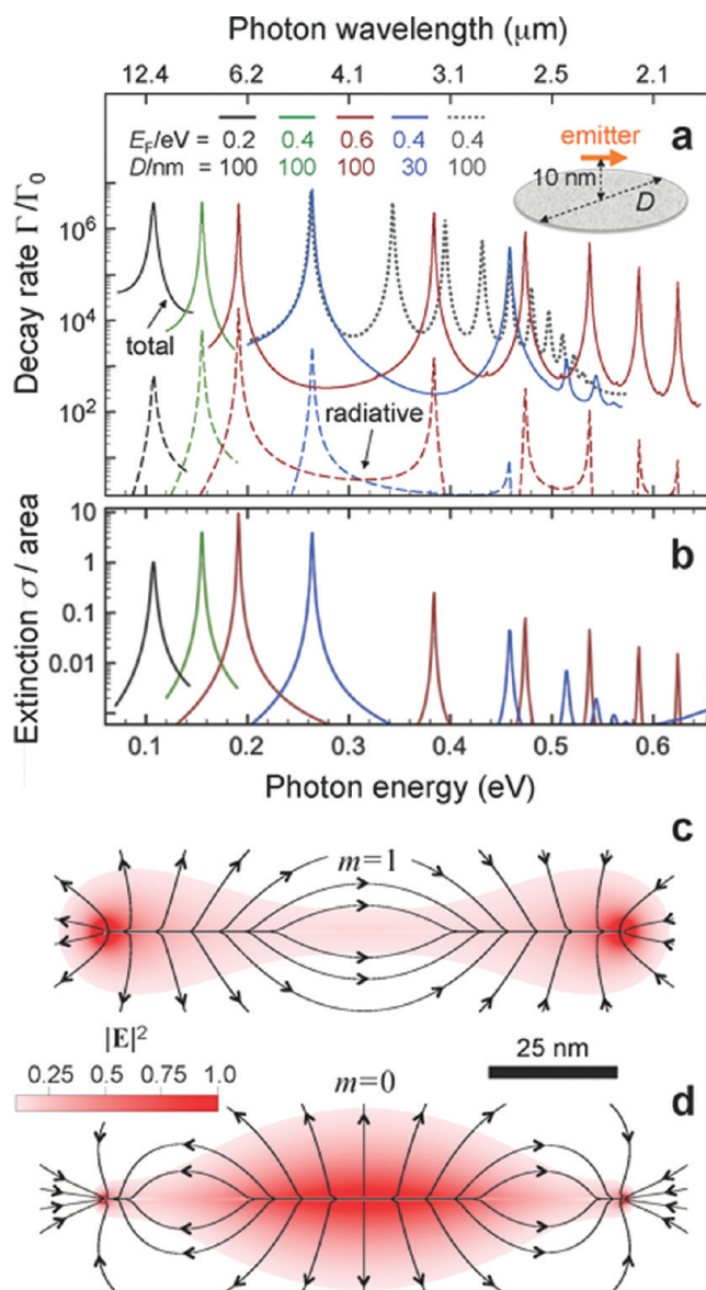
Figure 4. Plasmons in graphene nanodisks. (a) Decay rate of an emitter situated 10 nm above the center of a doped graphene disk for two different disk diameters D and various values of the Fermi energy E_F , as shown in the legend. Total decay rates (solid curves) are compared to the contribution of radiation emission (dashed curves). Some of the curves are only shown over a limited energy range for the sake of clarity. The emitter is polarized parallel to the disk, so that it excites SPs of m = 1 azimuthal symmetry, except in the dotted curve, corresponding to perpendicular orientation ( m = 0 symmetry) for D = 100 nm and E_F = 0.4 eV. (b) Normal-incidence extinction cross section of the same disks as in (a). (c, d) Near-electric-field intensity of the lowest-energy modes in a D = 100 nm disk doped to E_F = 0.4 eV for m = 0 ( \hbar\omega = 0.16 eV) and m = 1 ( \hbar\omega = 0.26 eV) azimuthal symmetries. Electric-field lines are superimposed on the intensity plot.
