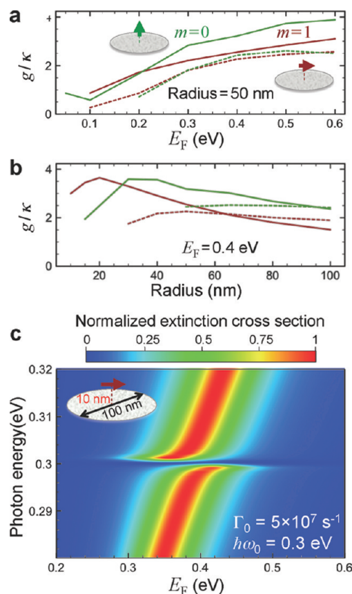
Figure 5. Strong coupling and vacuum Rabi splitting in graphene nanodisks. (a, b) Fermi-energy and disk-radius dependence of the strong-coupling parameter g/\kappa for an emitter placed 10 nm above the center of a doped graphene disk for the first-order (solid curves) and second-order (dashed curves) modes with either m = 0 (green curves) or m = 1 (red curves) azimuthal symmetries (the two lowest-order modes are shown for each symmetry). The natural decay rate of the emitter is \Gamma_0 = 5 \times 10^7 \text{ s}^{-1} (see eq 6 and below). (c) Fermi- and photon-energy dependence of the extinction cross section of a combined emitter–nanodisk system under the same conditions as in (a). The emitter has a resonance at \hbar\omega_0 = 0.3 \text{ eV} and is oriented parallel to the disk. The cross section is normalized to the maximum resonant extinction of the isolated disk.
