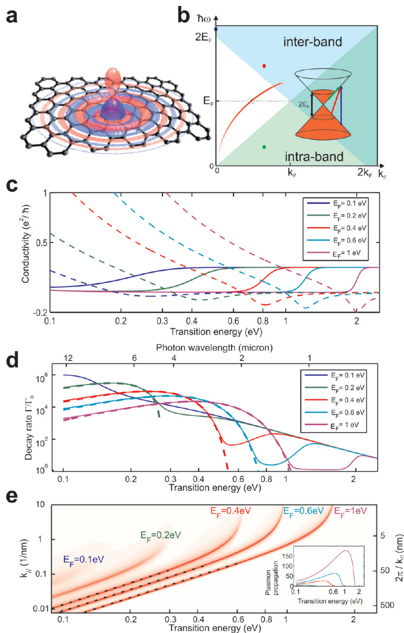
Figure 1. Coupling of a dipole emitter to doped homogeneous-graphene plasmons. (a) Near electric field produced by a perpendicular dipole situated 10 nm away from doped graphene. The photon and Fermi energies ( \hbar\omega and E_F ) are both 0.5 eV. The real (imaginary) part of the perpendicular electric field is shown as a red (blue) 3D contour. (b) Optical dispersion diagram showing the surface plasmon (SP) mode for E_F = 0.5 eV, as well as intra- and interband transitions in graphene. (c) Real (solid curves) and imaginary (dashed curves) parts of the conductivity of doped graphene. (d) Decay rate of an excited emitter in front of doped graphene as a function of photon emission energy for different values of E_F . The rate \Gamma is normalized to the free-space value \Gamma_0 . The emission dipole is perpendicular to the graphene and placed 10 nm away from it. Solid curves show the total decay rate, whereas dashed curves stand for the contribution of SP excitation. (e) Plasmon dispersion relation in doped graphene. The contour plot shows the Fresnel reflection coefficient |r_p| for various values of E_F . The dashed lines correspond to the Drude model (eq 2). The SP wave vector k_{sp} exhibits a quadratic dependence on plasmon energy. The inset shows the 1/e -amplitude-decay propagation distance 1/\text{Im}\{k_{sp}\} in units of the SP wavelength \lambda_{sp} = 2\pi/\text{Re}\{k_{sp}\} . The graphene is considered to lie on an \epsilon = 2 substrate in all cases.
